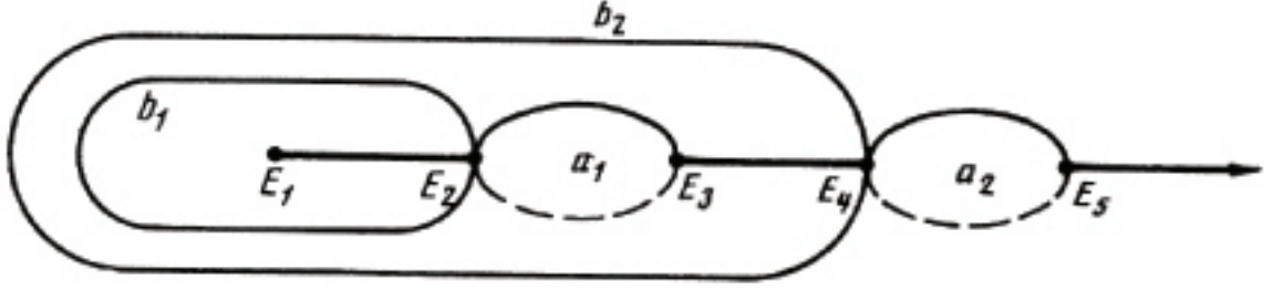
FIGURE 2. Basis of closed contours (cycles) on the Riemann surface R (two-band case). The cycles a_j correspond to forbidden bands while the part of the cycle a_j which lies on the lower sheet is shown by a dashed line.
